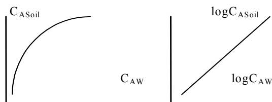
Fig. 2. Freundlich Adsorption Plot, normal and linearized
