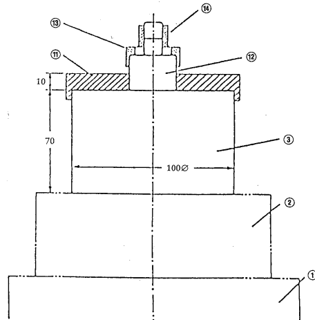
Fig. 4b Fall-hammer, lower part
