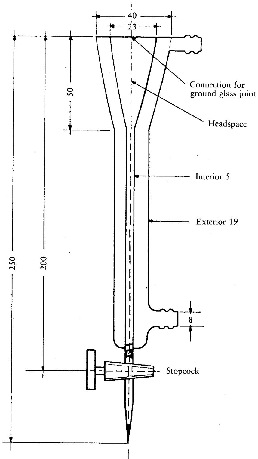
A typical microcolumn (All dimensions in millimetres)
